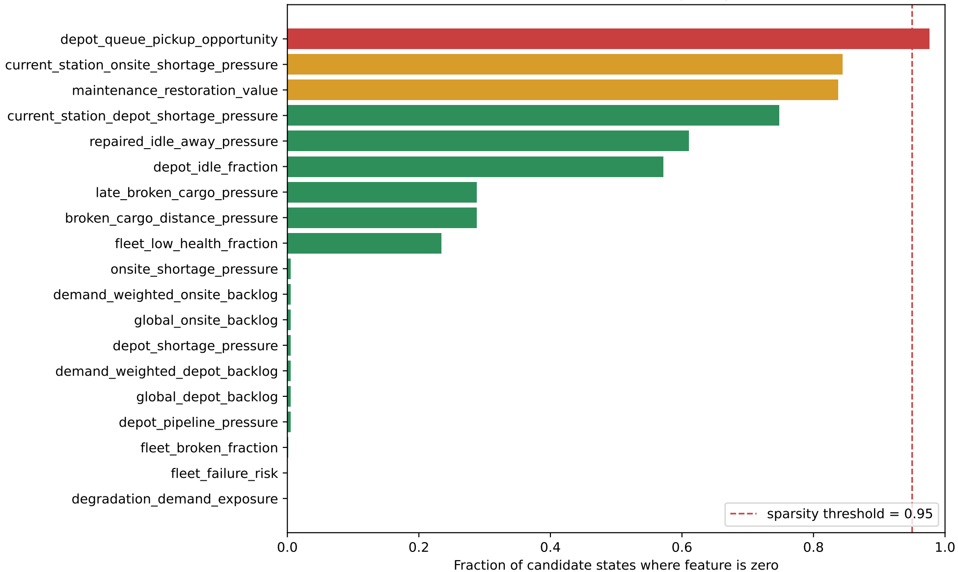
Maintenance Feature Sparsity
