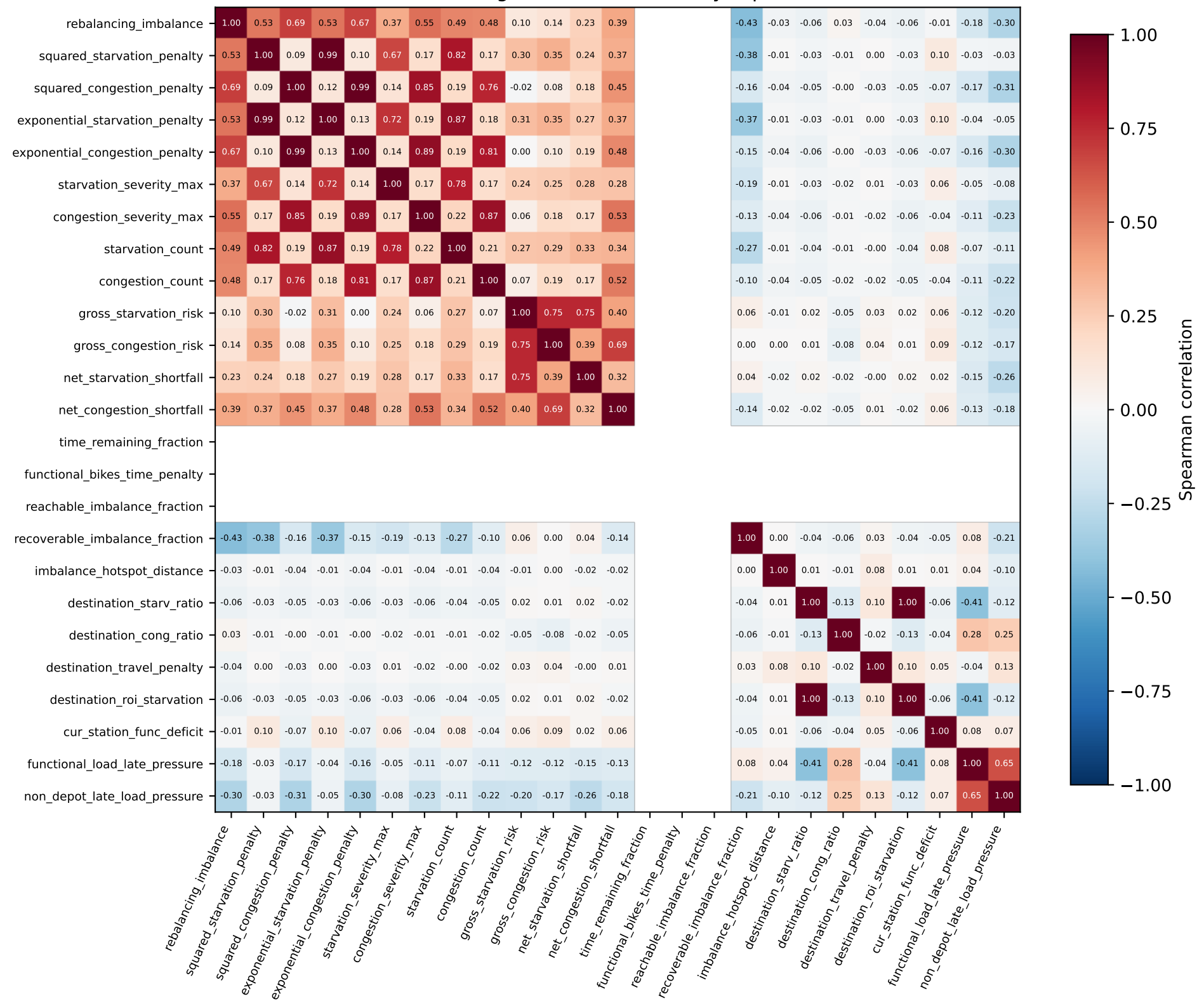
Rebalancing Feature Redundancy (Spearman)
