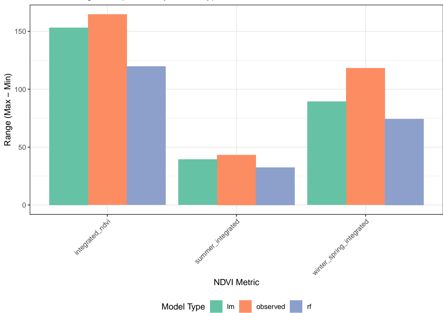
PLOTS: Range Comparison by Model Type
