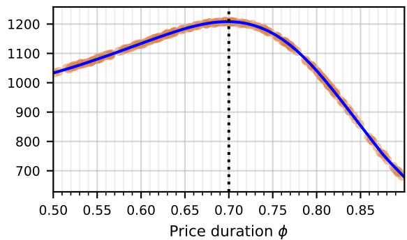
Log Likelihood \log \mathcal{L}_{\delta} conditioned on \phi_Y
