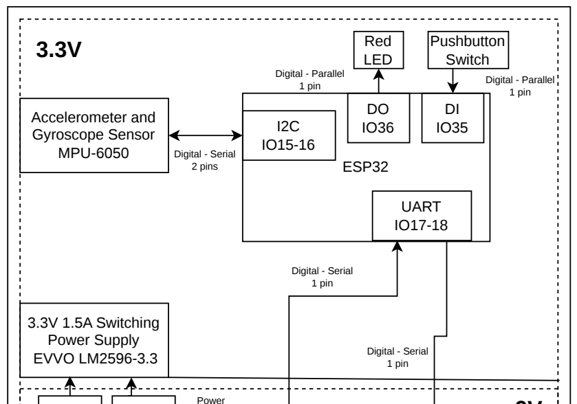
Block Diagram - Hafsa Kaysan Team 201 C3 Subsystem
