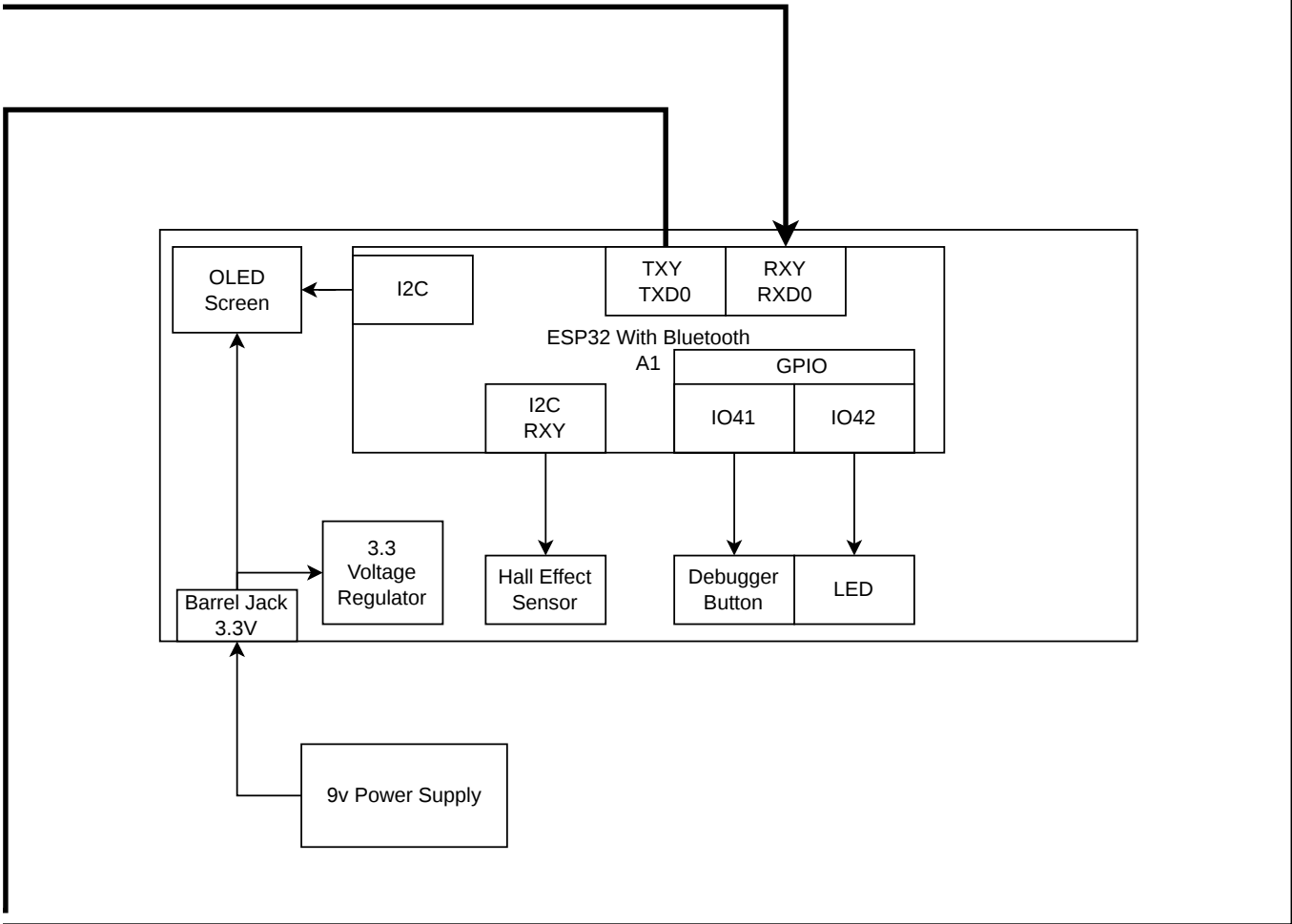
Block Diagram -- Team 201: EGR 314 Isaac Smith (A3)
