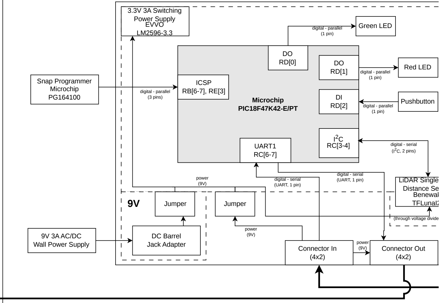
Block Diagram - Seth Merwin Team 201 - D2 Subsystem
