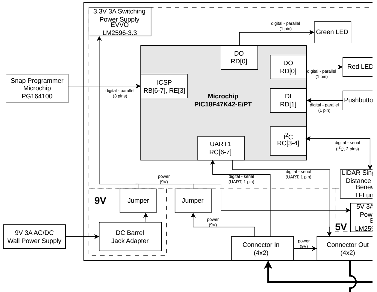
Block Diagram - Seth Merwin Team 201 - D2 Subsystem
