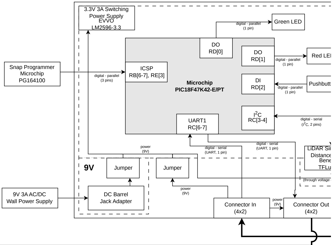
Block Diagram - Seth Merwin Team 201 - D2 Subsystem
