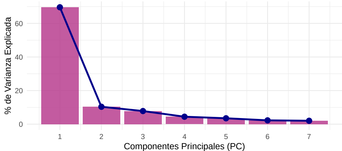
Scree Plot – Varianza Individual
