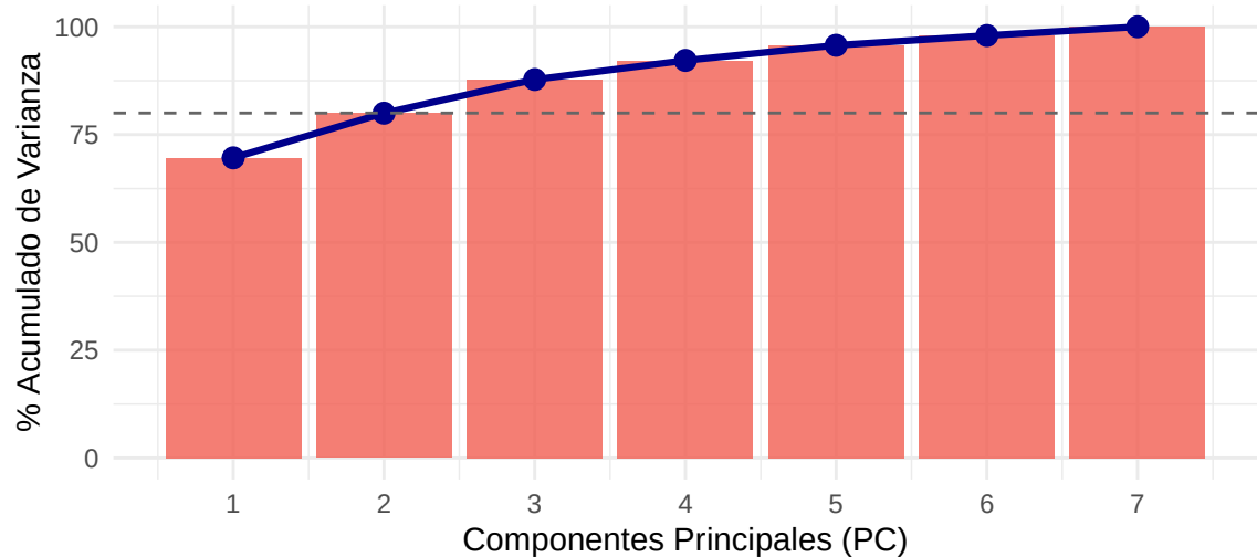
Scree Plot – Varianza Acumulada
