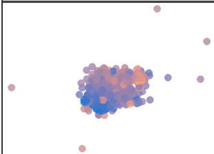
perplexity: 30
