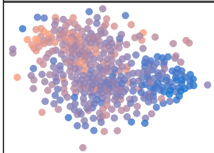
perplexity: 50
