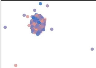
perplexity: 10
