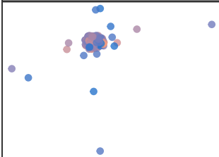
perplexity: 15
