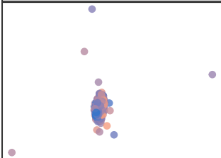
perplexity: 25
