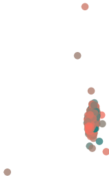
perplexity: 25
