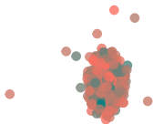
perplexity: 10
