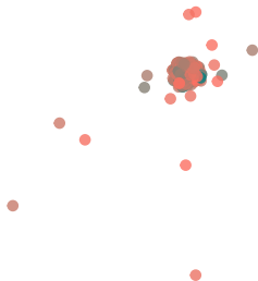
perplexity: 15
