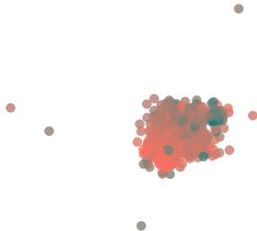
perplexity: 30
