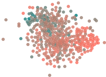
perplexity: 50
