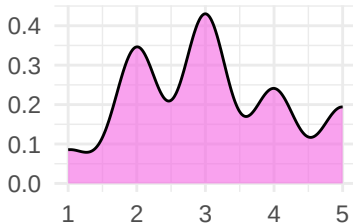
University.Rating
