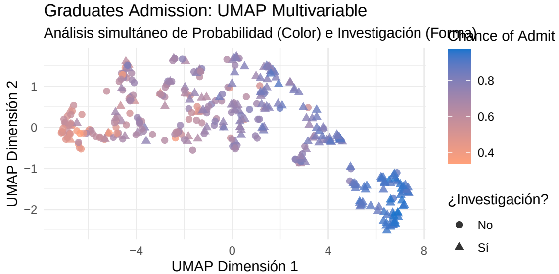
Figura 15: UMAP multivariable: color = Chance of Admit, forma = Research
