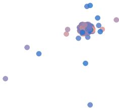
perplexity: 15
