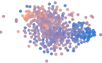
perplexity: 50
