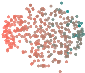
perplexity: 50
