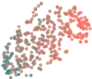
perplexity: 30
