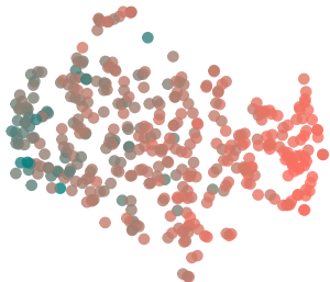
perplexity: 25
