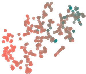
perplexity: 10
