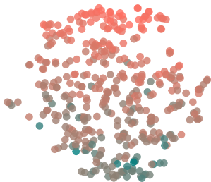
perplexity: 20
