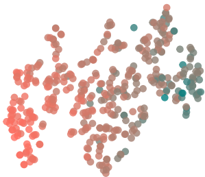
perplexity: 15
