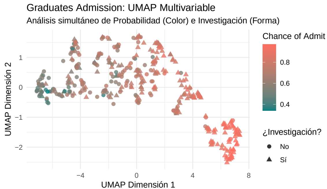
Figura 12: UMAP multivariable: color = Chance of Admit, forma = Research
