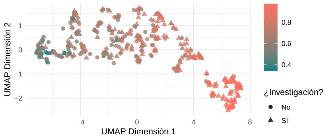
Figura 10: UMAP multivariable: color = Chance of Admit, forma = Research
