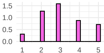
University.Rating
