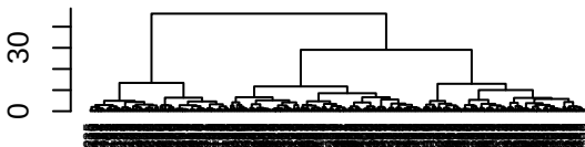
Linkage: ward.D2
