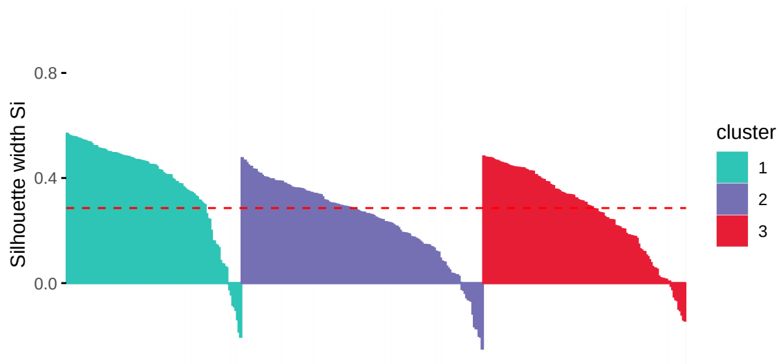
Clusters silhouette plot Average silhouette width: 0.29
