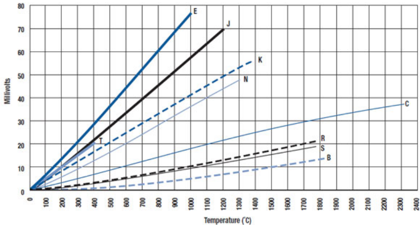
Thermocouple EMF Versus Temperature
