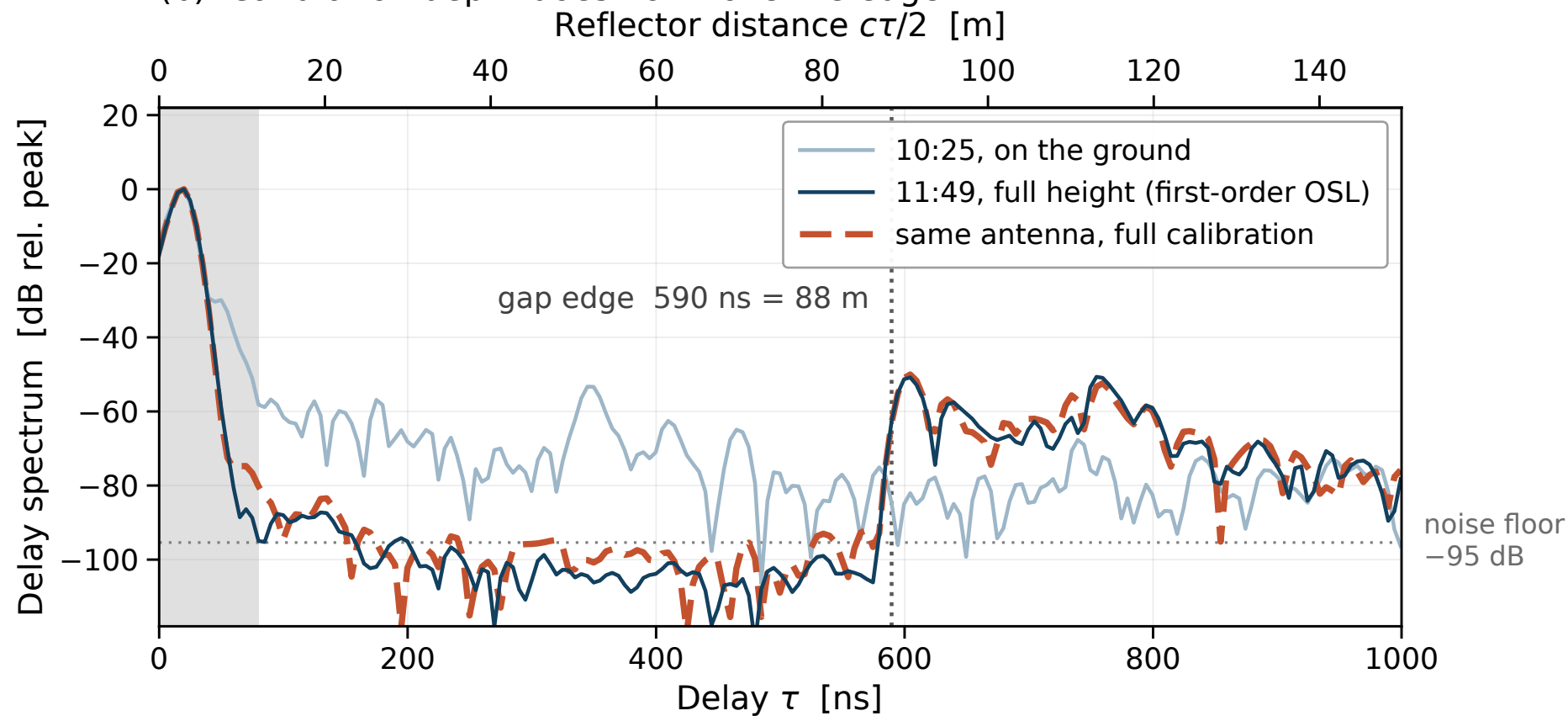
(b) Calibration depth does not move the edge
