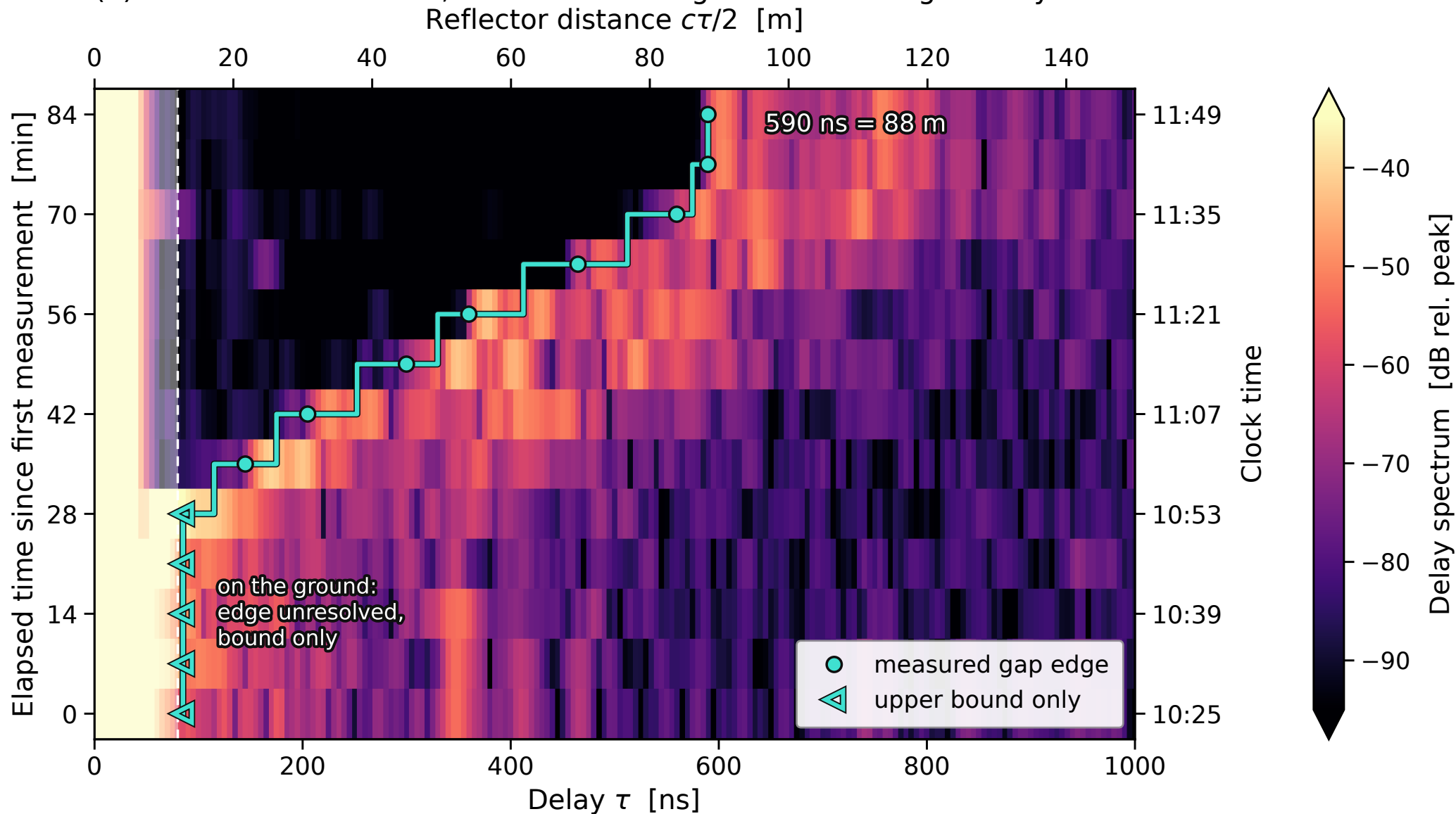
(a) As the antenna rises, the reflection edge moves to longer delay
