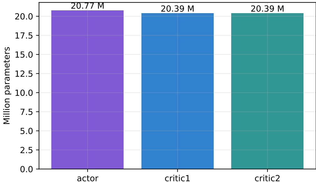
Round-32 actor/critic parameter allocation
