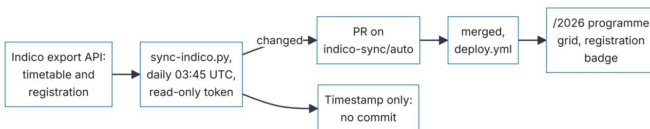
Figure 7 · The Indico pipeline. Without its token the sync runs in anonymous mode and still carries the public timetable, so an expired token degrades the site rather than breaking it.
