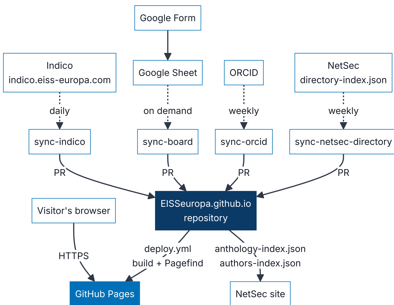
Figure 2 · End-to-end stack. Solid lines are requests and pushes, dashed lines are scheduled or on-demand sync jobs. Every sync lands as a pull request, never as a direct push to master .
