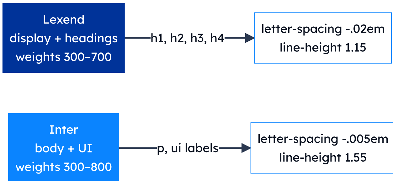
Figure 8 · Type pairing. Lexend's high x-height makes for friendly, fast-reading headlines; Inter is the most-tested body face for UI at small sizes.
