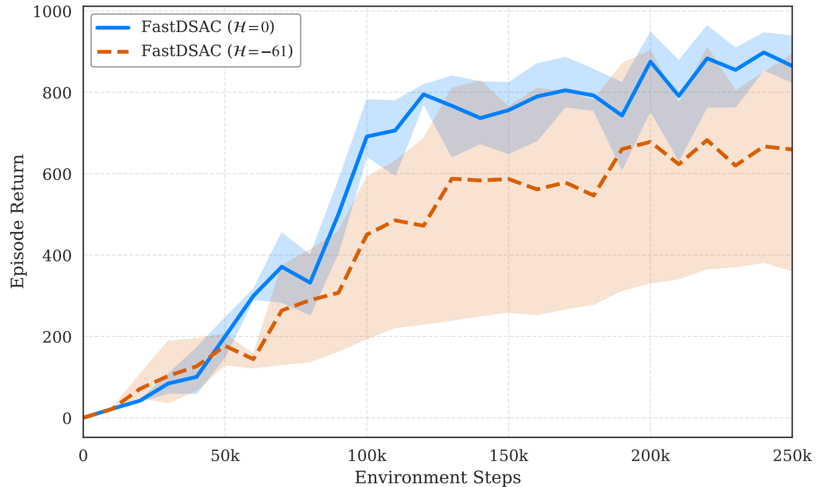
Basketball Target Entropy Comparison
