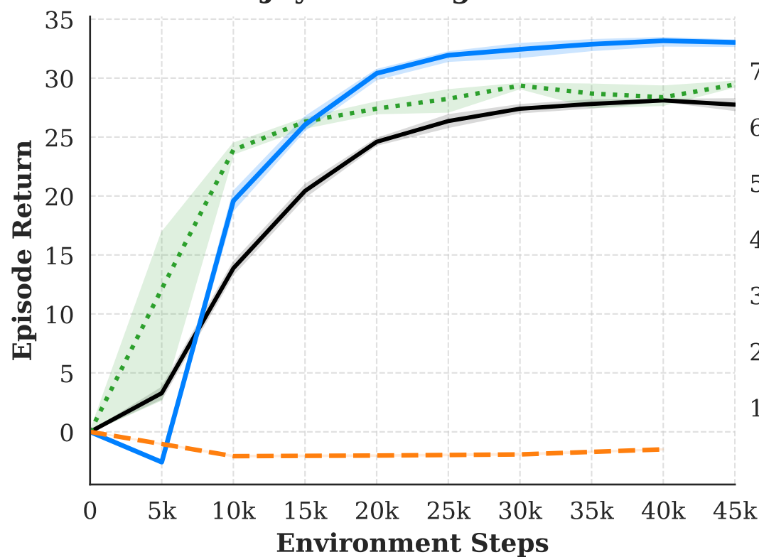
Isaac-Velocity-Rough-H1-v0
