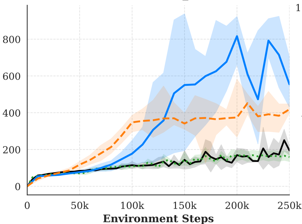
h1hand-stair-v0
