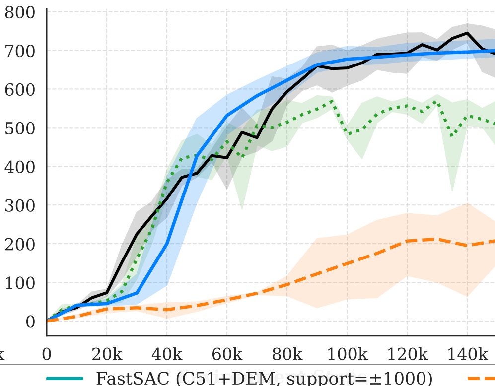
h1hand-stair-v0
