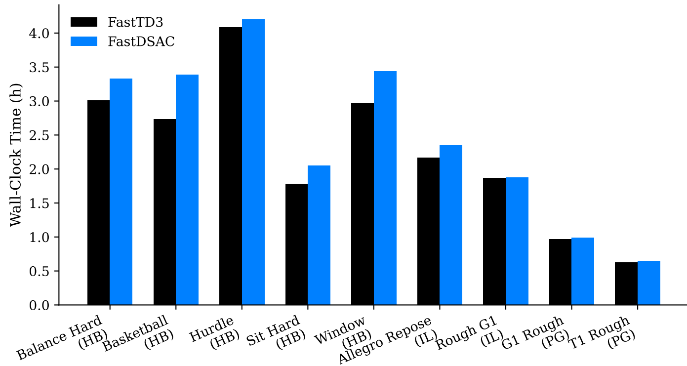
Wall-Clock Time Comparison
