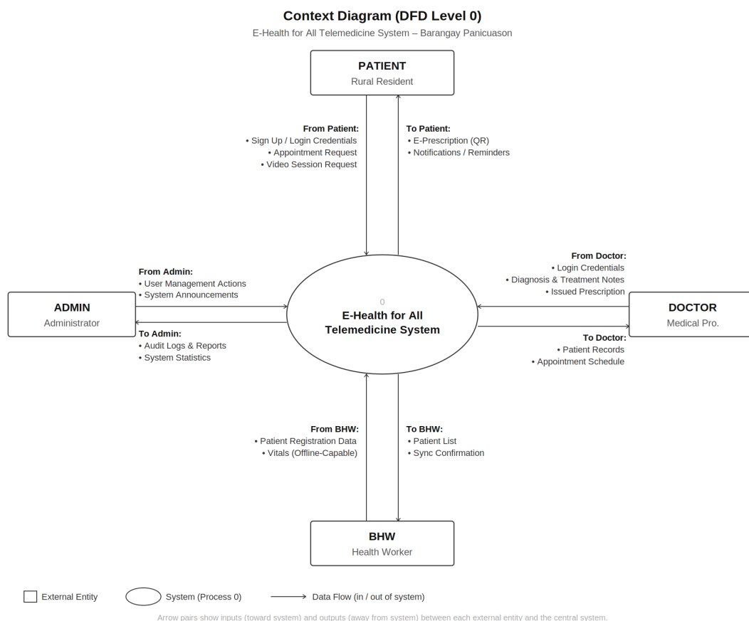
Figure 2.3: DFD Level 0
