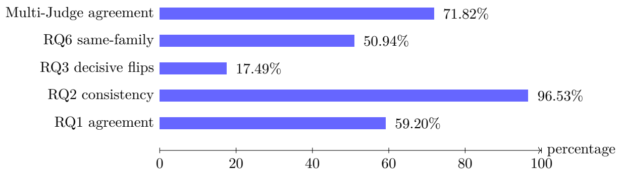
Figure 5.1: Selected final percentages. Metrics measure different estimands and are not a common score or ranking.
