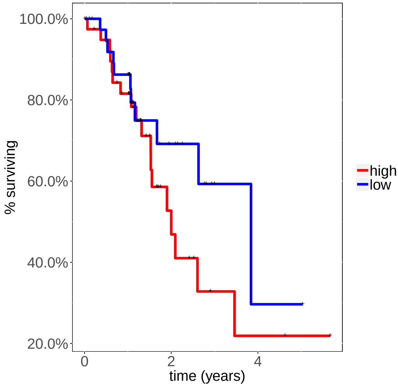
ESCA BAK1 Logrank p-value=0.225159
