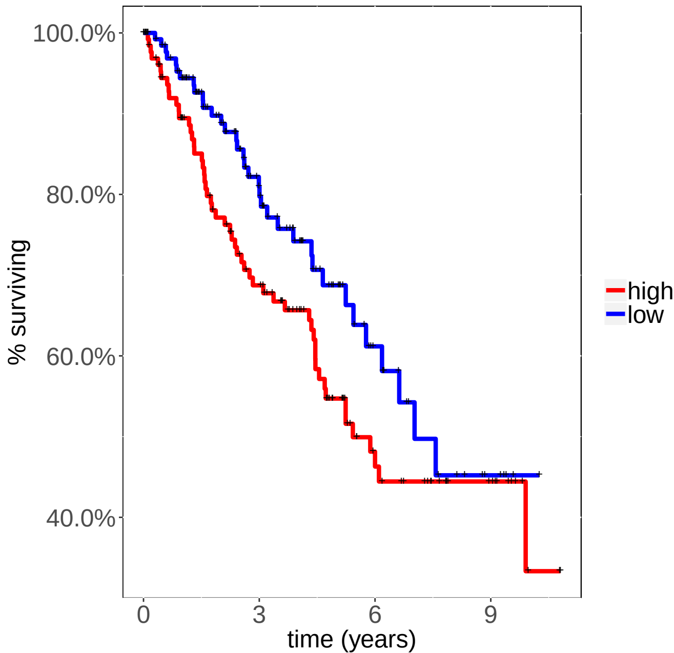
KIRC BAK1 Logrank p-value=0.0770319
