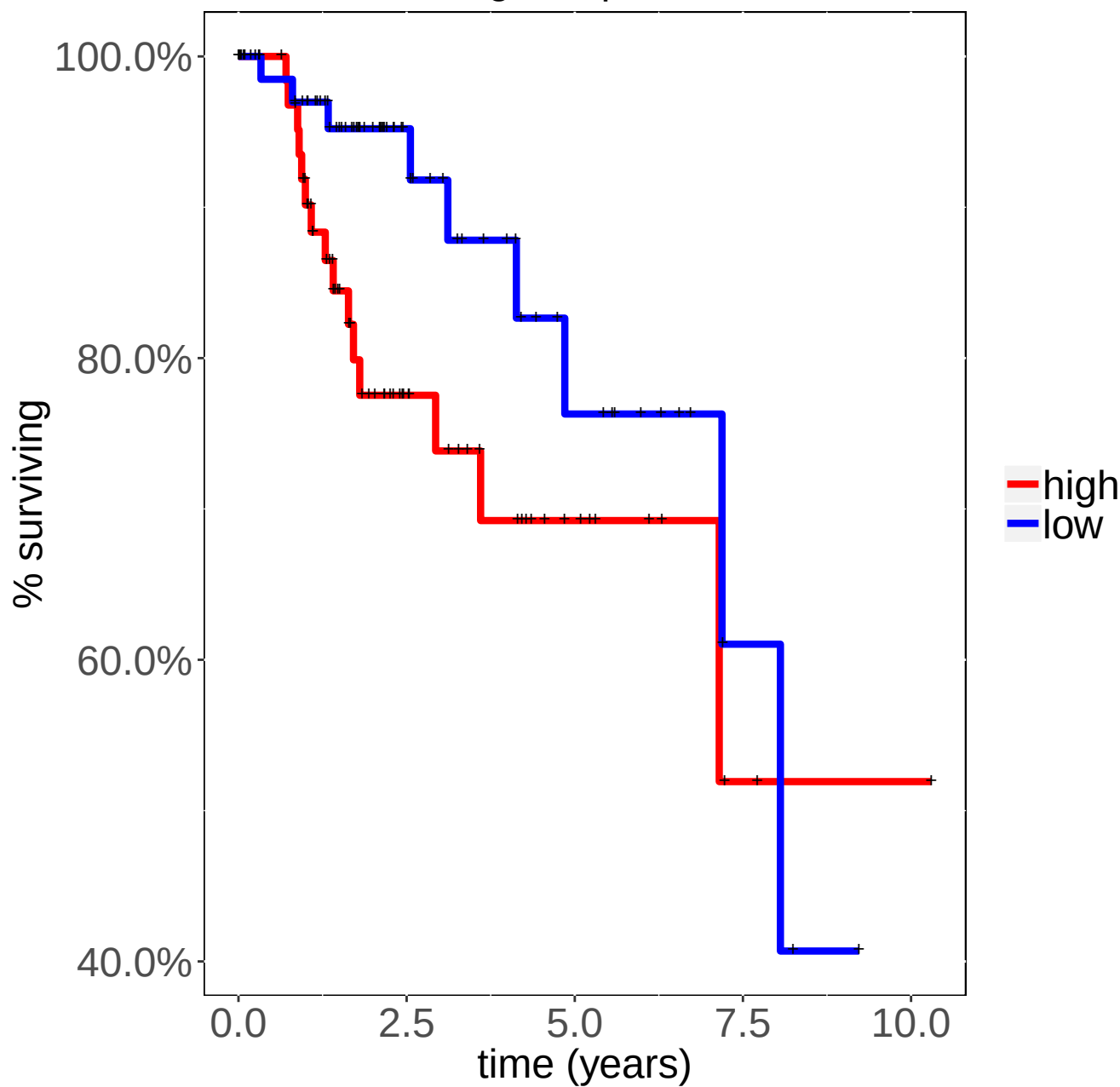
KIRP BAK1 Logrank p-value=0.0764076
