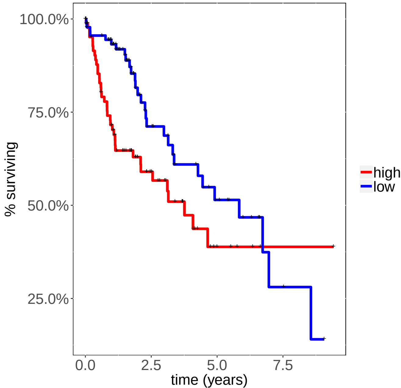
LIHC BAK1 Logrank p-value=0.0191652
