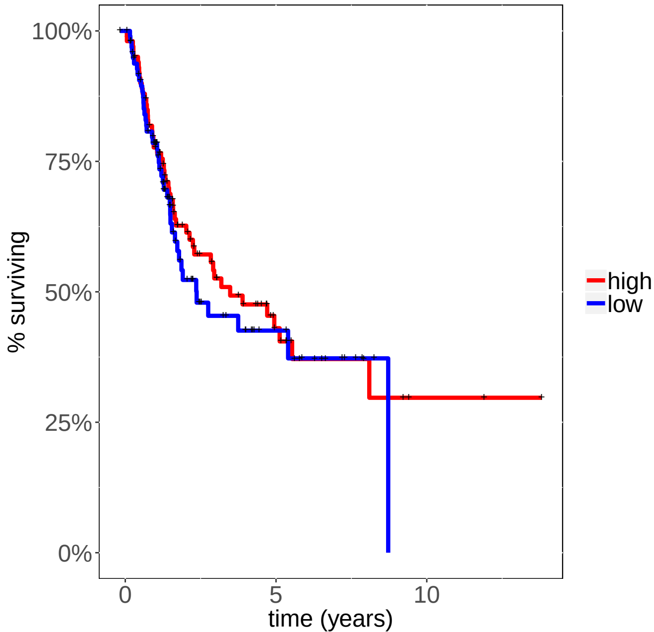
BLCA BAX Logrank p-value=0.517904
