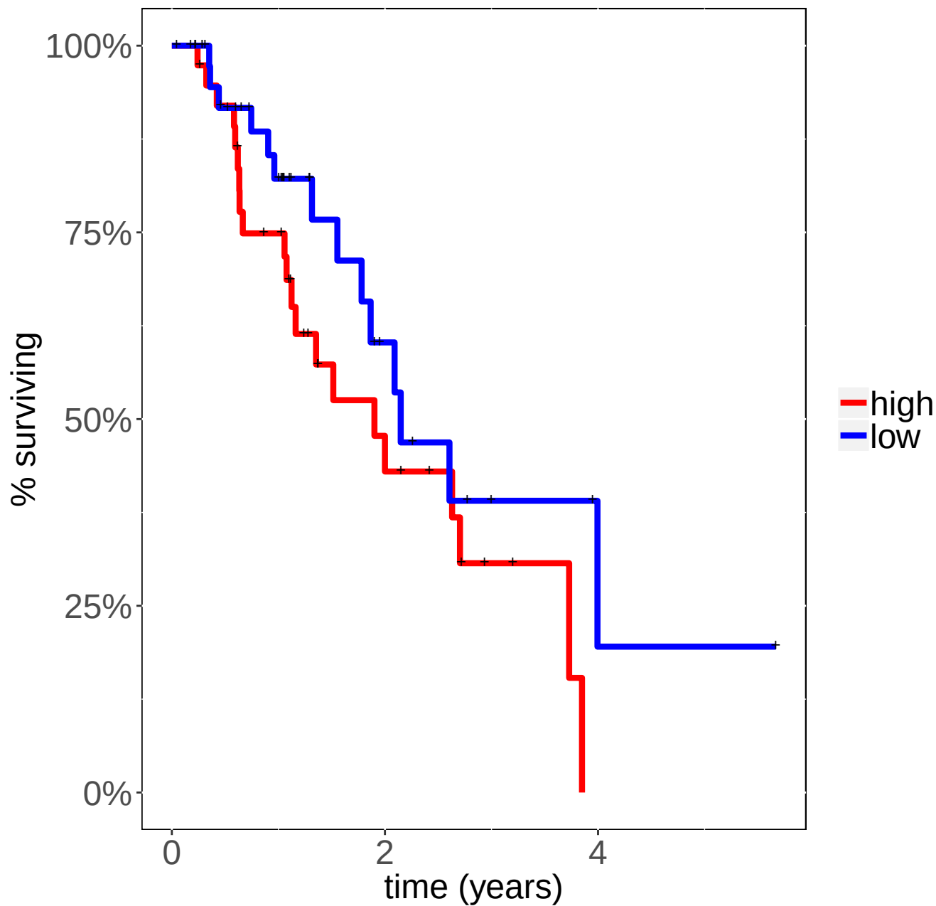
ESCA BAX Logrank p-value=0.140861
