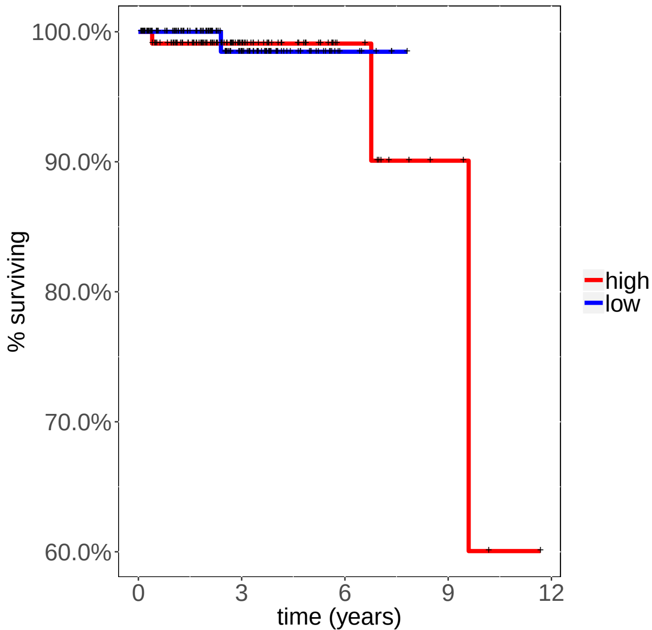
PRAD BAX Logrank p-value=0.74927
