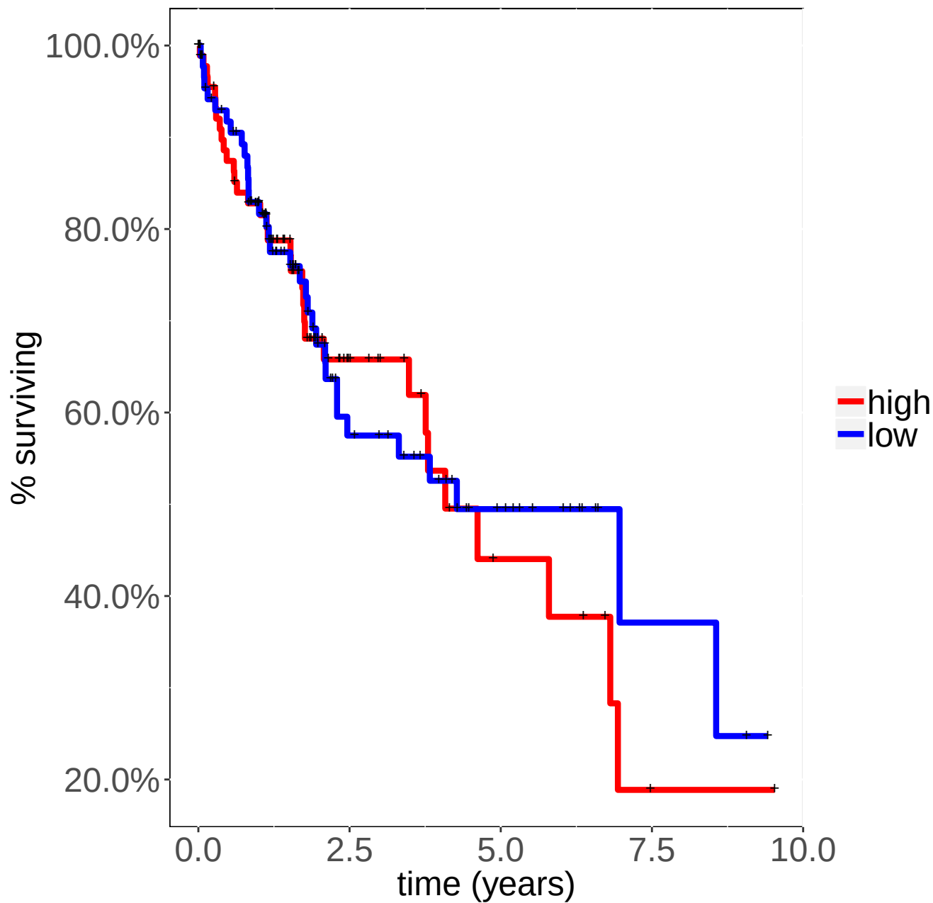
LIHC BCL2A1 Logrank p-value=0.767059
