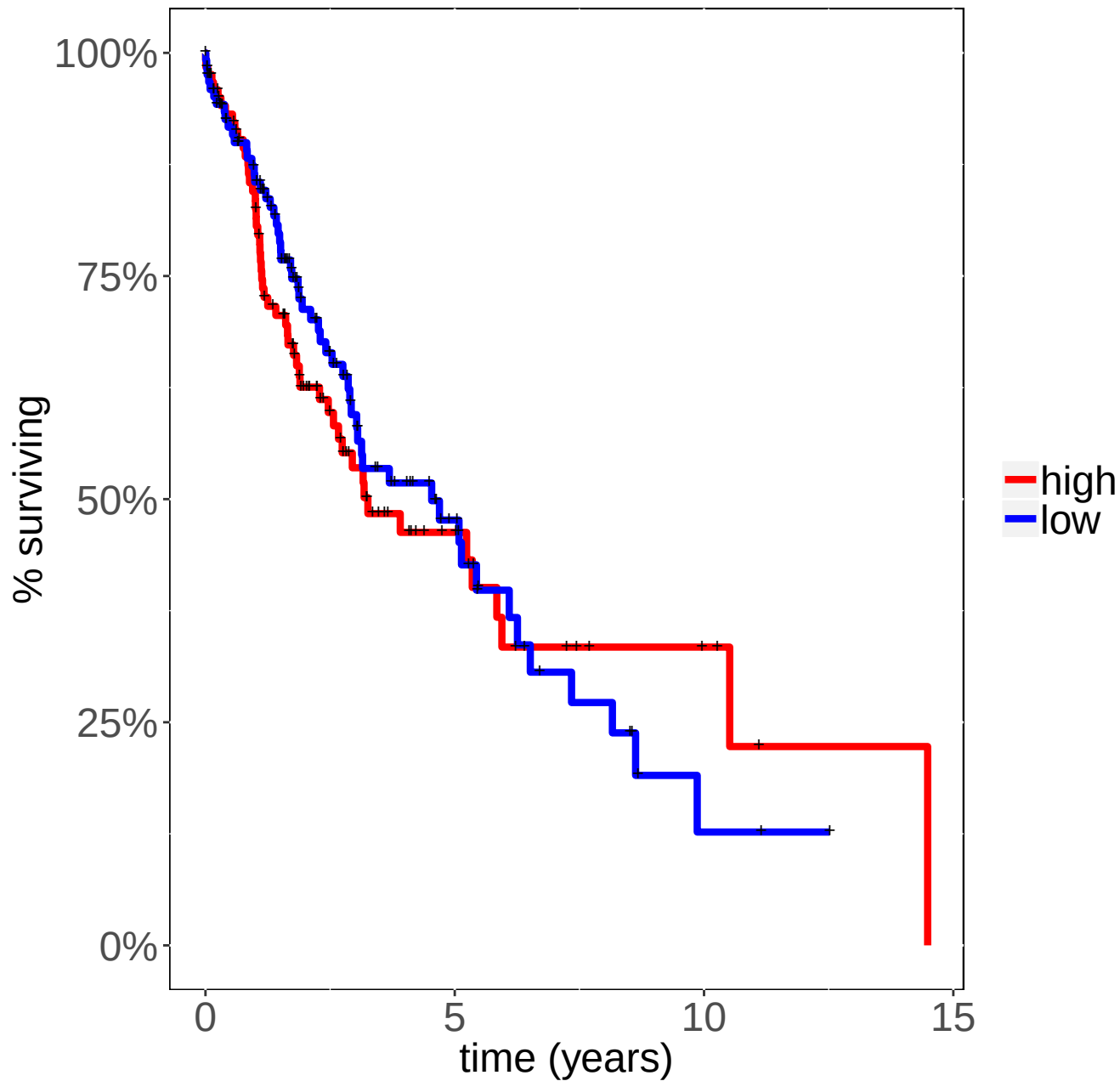
LUSC BCL2A1 Logrank p-value=0.707701
