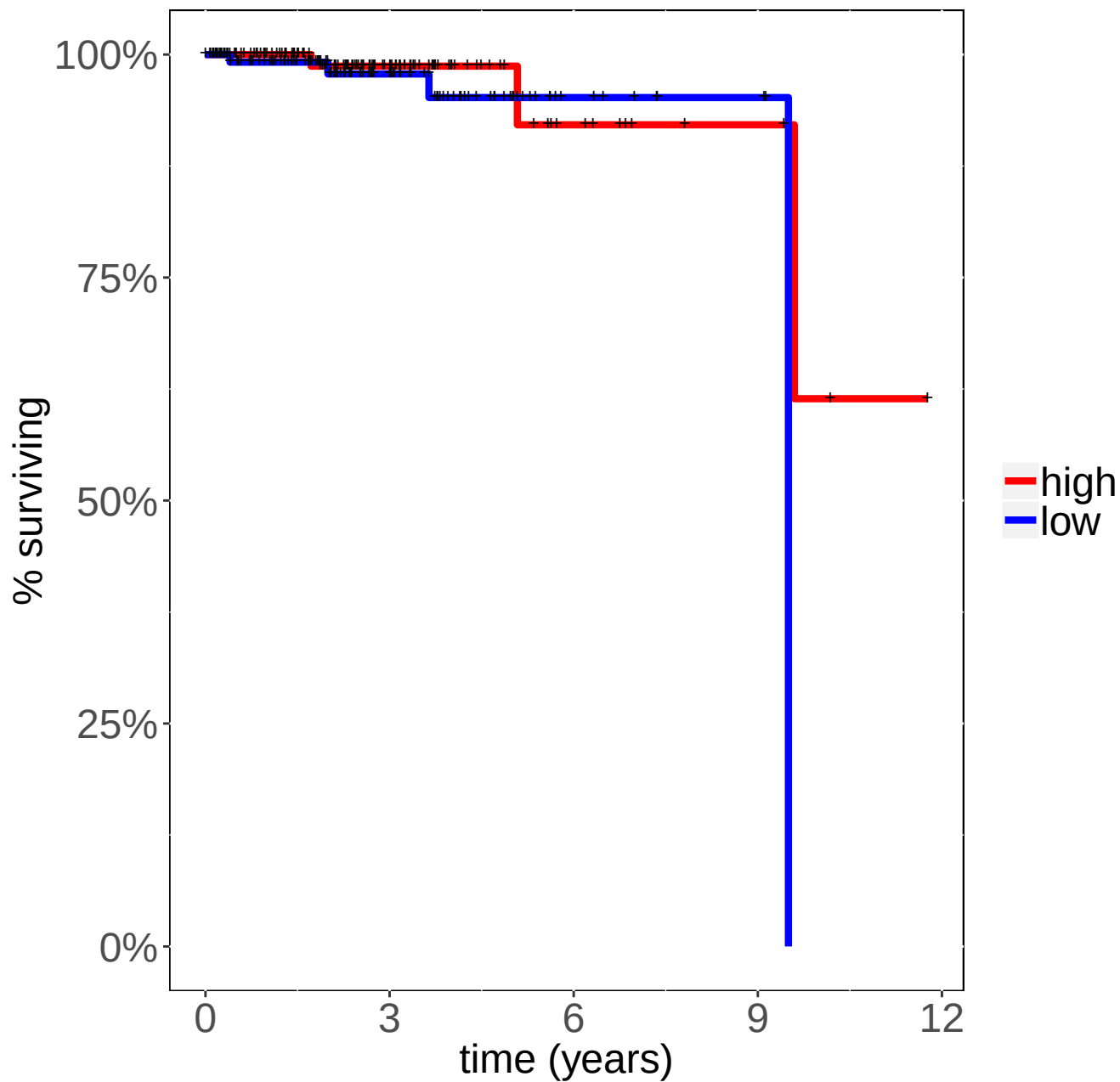
PRAD BCL2A1 Logrank p-value=0.33352
