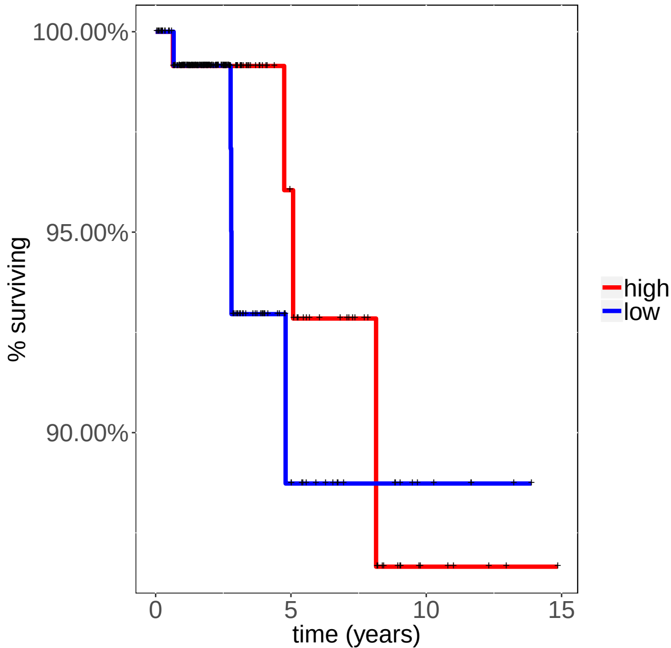
THCA BCL2A1 Logrank p-value=0.502943
