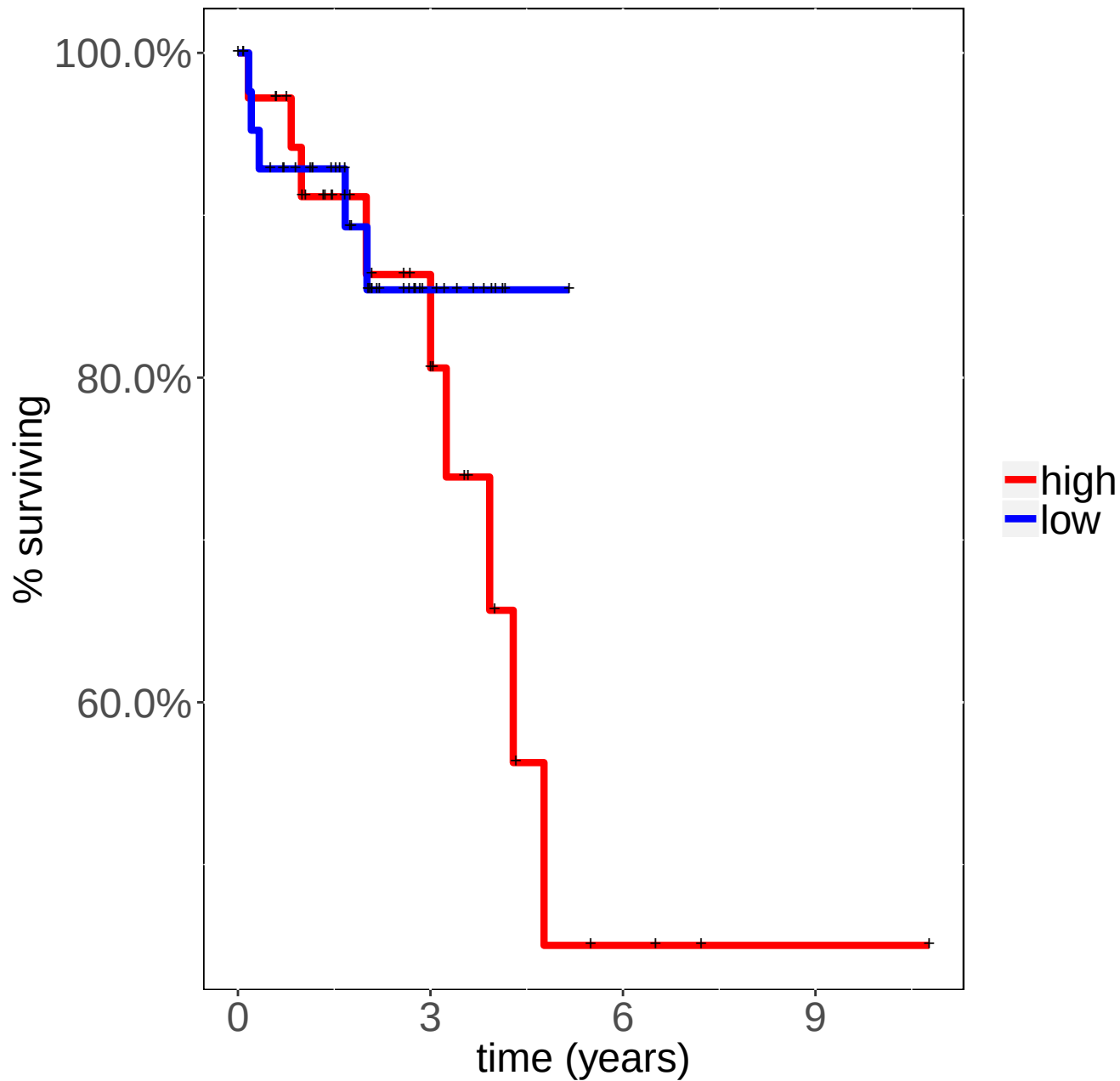
READ BCL2L1 Logrank p-value=0.458264
