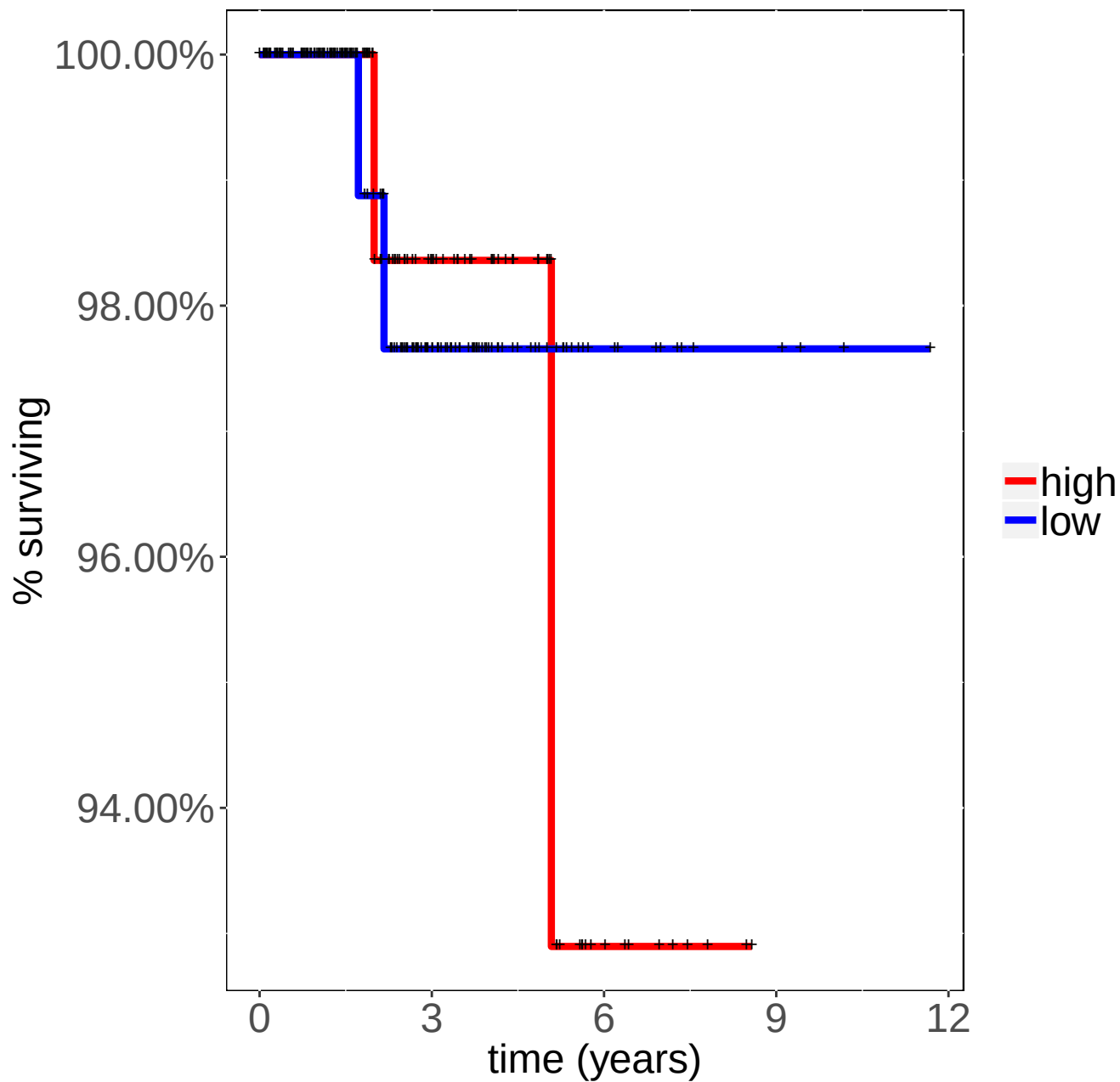
PRAD BCL2L2 Logrank p-value=0.814958
