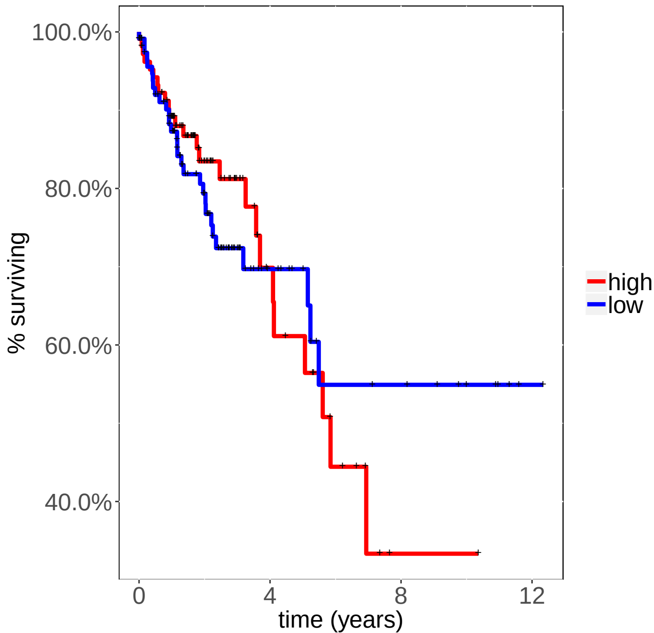
COAD BCL2 Logrank p-value=0.89435
