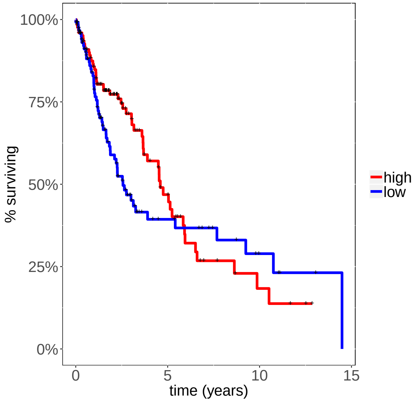
LUSC BCL2 Logrank p-value=0.170267
