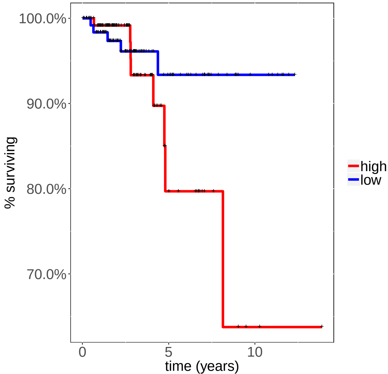
THCA BCL2 Logrank p-value=0.16159
