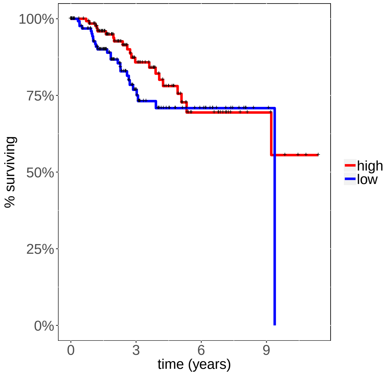
UCEC BCL2 Logrank p-value=0.141656
