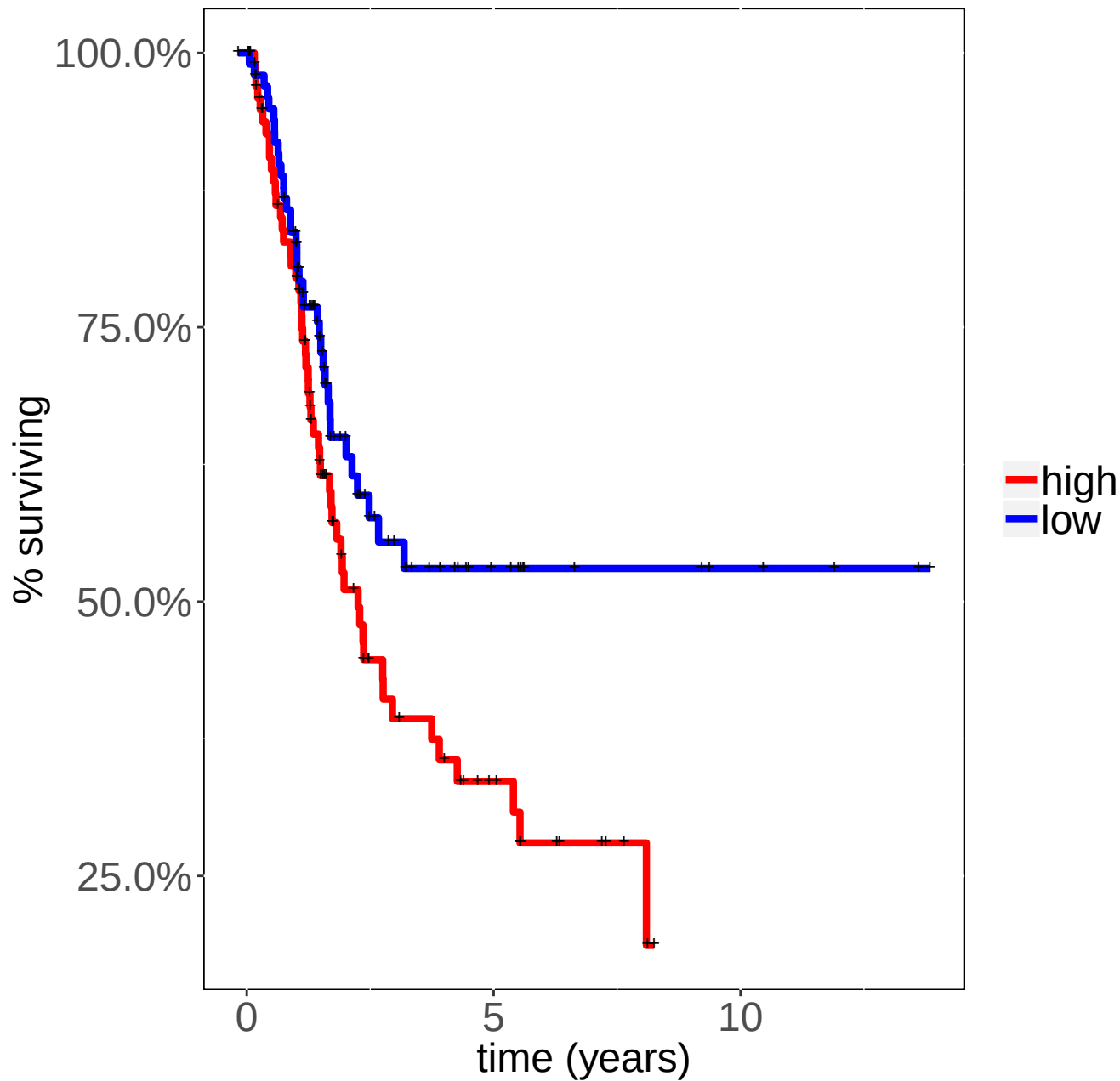
BLCA BOK Logrank p-value=0.0279273
