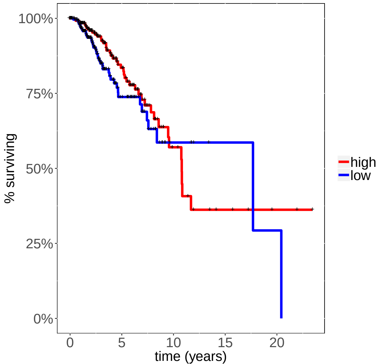
BRCA BOK Logrank p-value=0.195295
