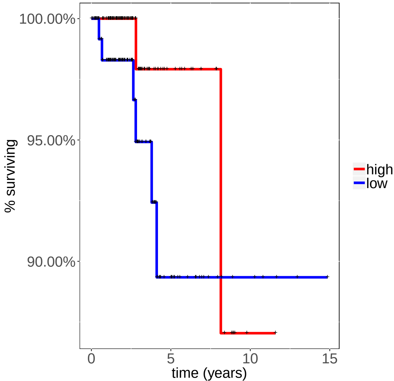
THCA BOK Logrank p-value=0.196295
